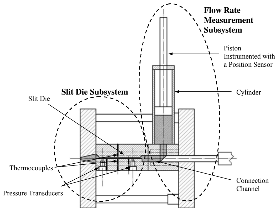
Figure 3. Scheme of the in-line rheometer
