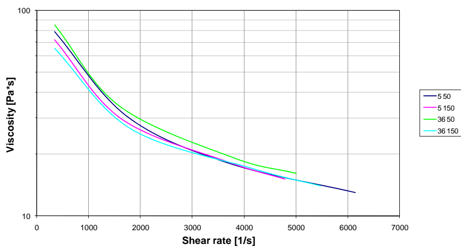
Figure 4. Apparent viscosity curves for various conditions of plastification.
