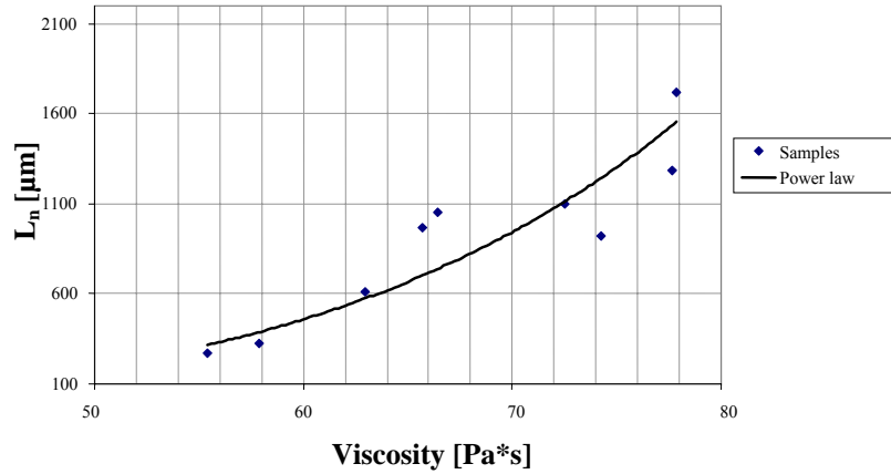
Figure 6. Correlation between the viscosity measures and the number-averaged lengths.
