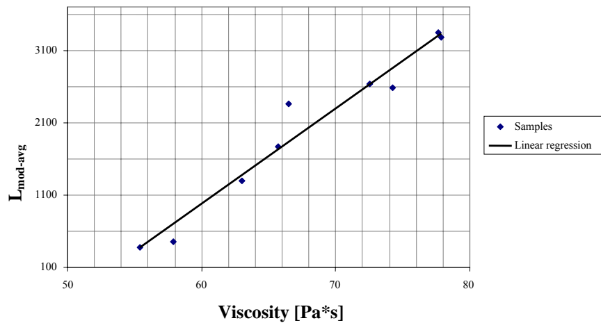
Figure 7. Correlation between the viscosity measures and the average lengths according to Huq and Azaiez.
