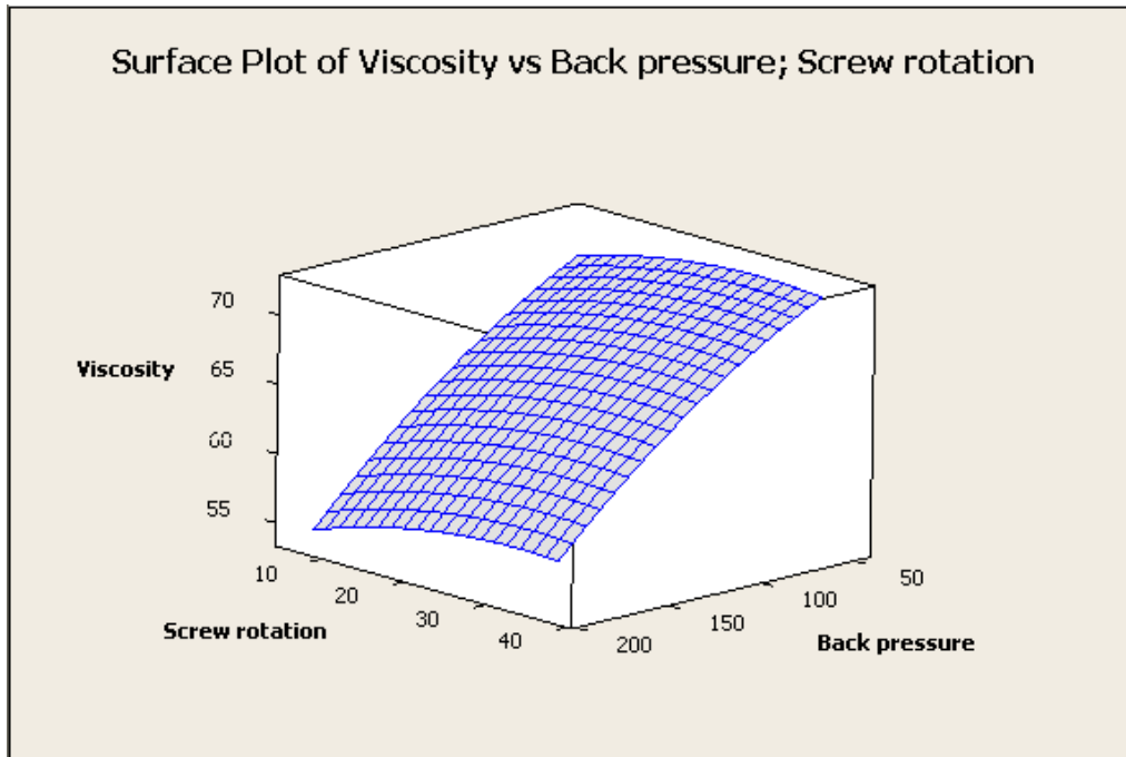
Figure 8. Response surface for viscosity.
