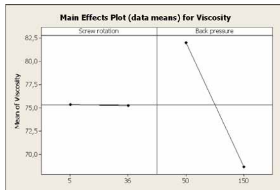
Figure 5. Effects plot for the viscosity measurements.
