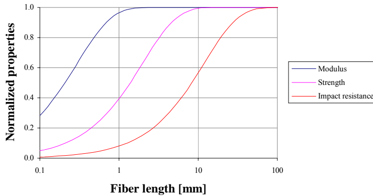
Figure 1. Qualitative relation between the normalized mechanical properties and the fiber length of a glass fiber reinforced PP (fiber diameter = 10 \mu\text{m} ).
